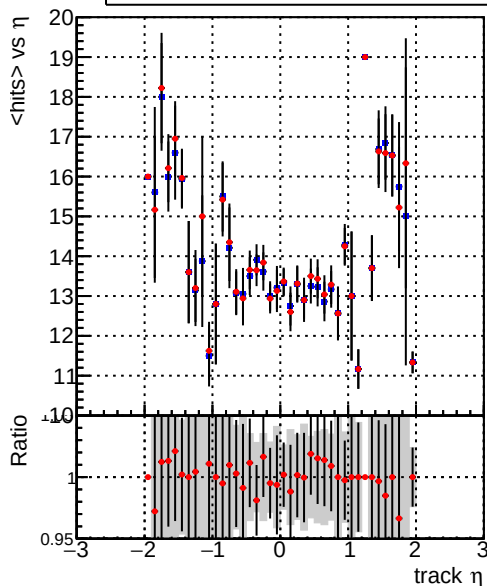
mean hit — DQM_CKF_TTbase — DQM_CKF_TT_retrainOldFiles125_v2_prelimWP_epoch4
