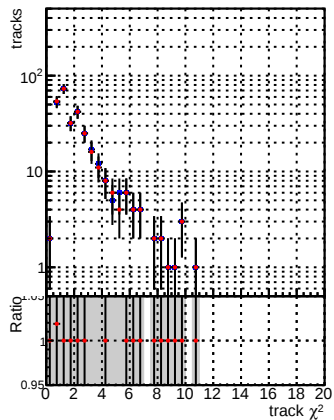
N of reco track vs. \chi^2 for DQM CKF TTbase and DQM CKF TT_retrainOldFiles125_v2_prelimWP_epoch4
