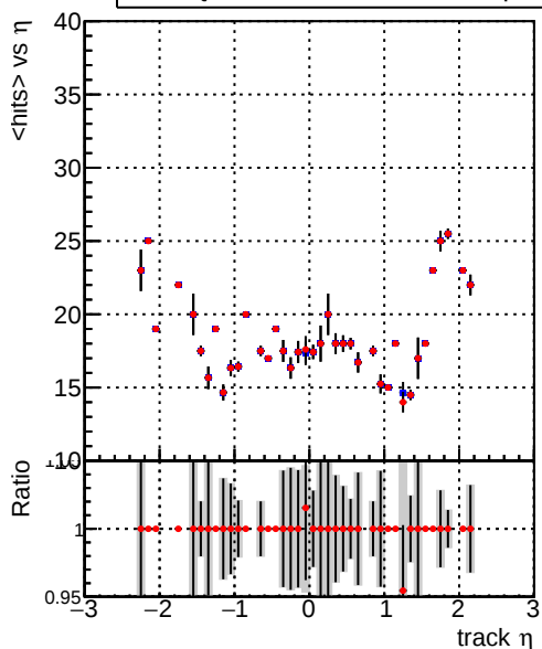
mean hits vs \eta Legend: DQM_CKF_TTbase (blue line with dots), DQM_CKF_TT_retrainOldFiles125_v2_prelimWP_epoch4 (red line with dots)
