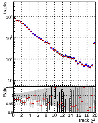
N of reco track vs. \chi^2 —●— DOM_CKF_TTbase —●— DOM_CKF_TT_retrainOldFiles125_v2_prelimWP_epoch4
