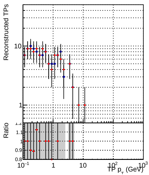
Legend: DQM_CKF_TTbase (blue dots), DQM_CKF_TT_retrainOldFiles125_v2_prelimWP_epoch4 (red dots)
