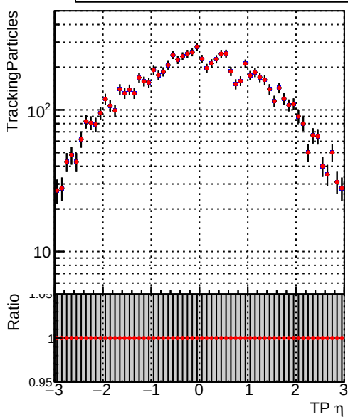
N of simulated tracks vs \eta Legend: DQM_CKF_TTbase (blue diamonds), DQM_CKF_TT_retrainOldFiles125_v2_prelimWP_epoch4 (red diamonds)
