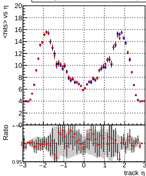
— DQM_CKF_TTbase — DQM_CKF_TT_retrainOldFiles125_v2_prelimWP_epoch4 mean hits vs \eta
