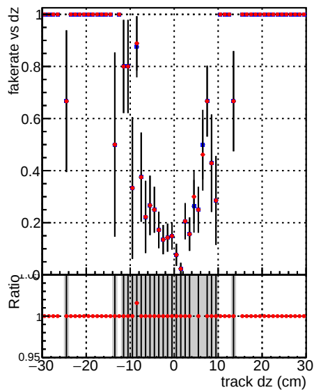
Fake rate vs dz —●— DQM_CKF_TTbase —●— DQM_CKF_TT_retrainOldFiles125_v2_prelimWP_epoch4
