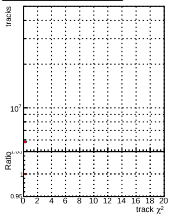
N of reco track vs. \chi^2 —●— DOM_CKF_TTbase —●— DOM_CKF_TT_retrainOldFiles125_v2_prelimWP
