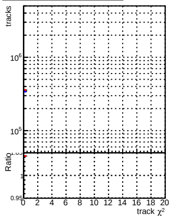
N of reco track vs. \chi^2 —•— DQM_CKF_TTbase —•— DQM_CKF_TT_retrainOldFiles125_v2_prelimWP
