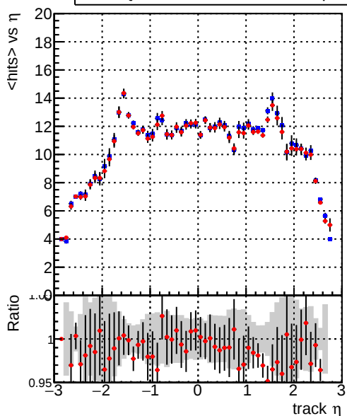
— DQM_CKF_TTbase — DQM_CKF_TT_retrainOldFiles125_v2_prelimWP mean hits vs \eta
