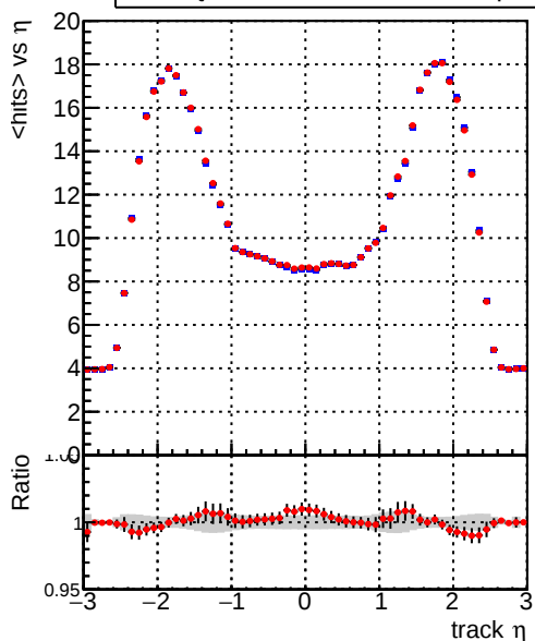
mean hits vs \eta — DQM_CKF_TTbase — DQM_CKF_TT_retrainOldFiles125_v2_prelimWP
