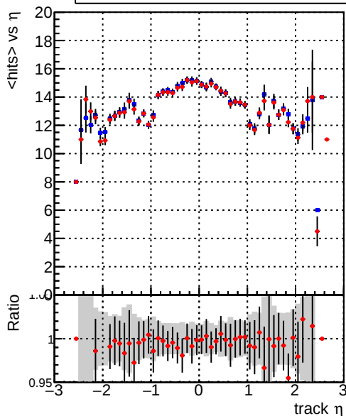
mean hits — DQM_CKF_TTbase — DQM_CKF_TT_retrainOldFiles125_v2_prelimWP
