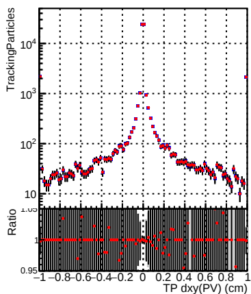
N of sim DQM_CKF_TT_retrainOldFiles125_v2_prelimWP
