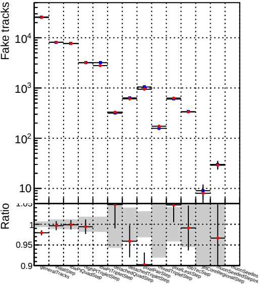
Number 1 DQM_CKF_TT_retrainOldFiles125_v2_prelimWP
