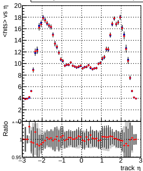
mean hits vs \eta Legend: DQM_CKF_TTbase (blue line), DQM_CKF_TT_retrainOldFiles125_v2_prelimWP (red line)
