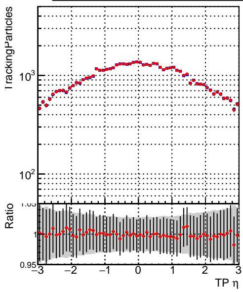
N of simulated tracks vs \eta Legend: DQM_CKF_TTbase (blue dots), DQM_CKF_TT_retrainOldFiles125_v2_prelimWP (red dots)
