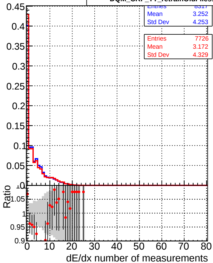
—■— DQM_CKF_TTbase —●— DQM_CKF_TT_retrainOldFiles125_v2_prelimWP
