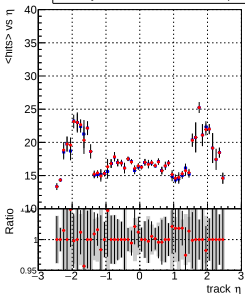
mean hits vs \eta Legend: DQM_CKF_TTbase (blue line with markers), DQM_CKF_TT_retrainOldFiles125_v2_prelimWP (red line with markers)
