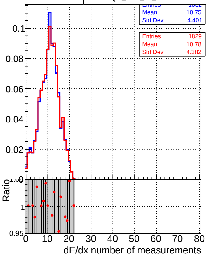
—■— DQM_CKF_TTbase —●— DQM_CKF_TT_retrainOldFiles125_v2_prelimWP
