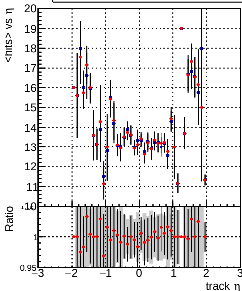
mean hit — DQM_CKF_TTbase — DQM_CKF_TT_retrainOldFiles125_v2_prelimWP
