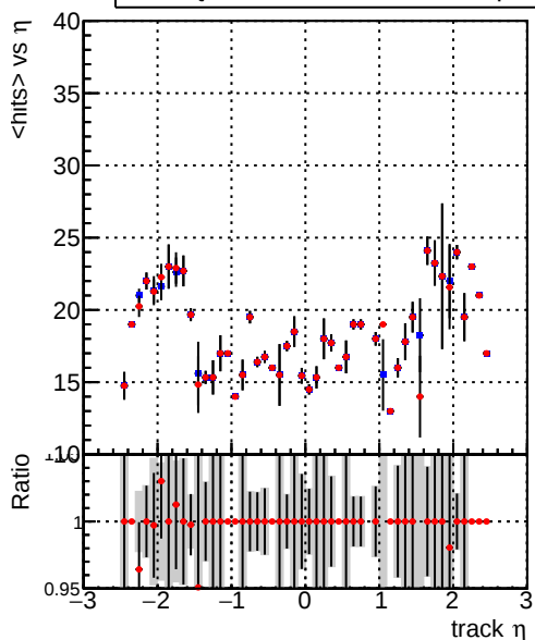
mean hit Legend: DQM_CKF_TTbase (blue line), DQM_CKF_TT_retrainOldFiles125_v2_prelimWP (red line)
