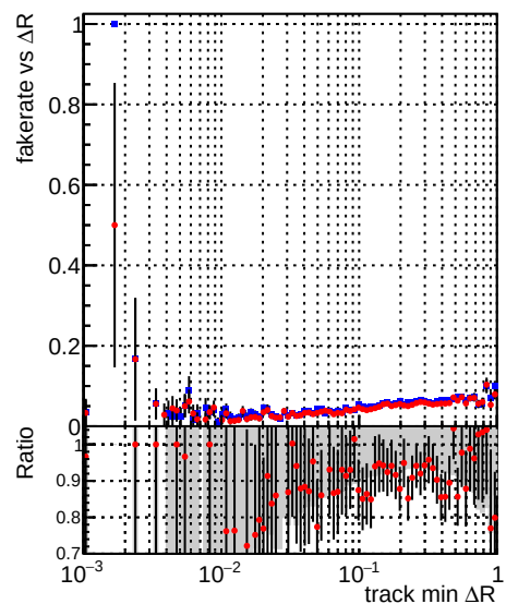
■ DQM_CKF_TTbase ● DQM_CKF_TT_retrainOldFiles125_v2_prelimWP
