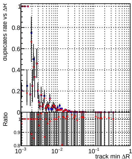
■ DQM_CKF_TTbase ● DQM_CKF_TT_retrainOldFiles125_v2_prelimWP
