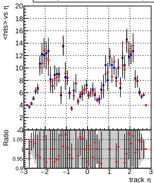
mean hit Legend: DQM_CKF_TTbase (blue line with circles), DQM_CKF_TT_retrainOldFiles125_v2_prelimWP (red line with circles)
