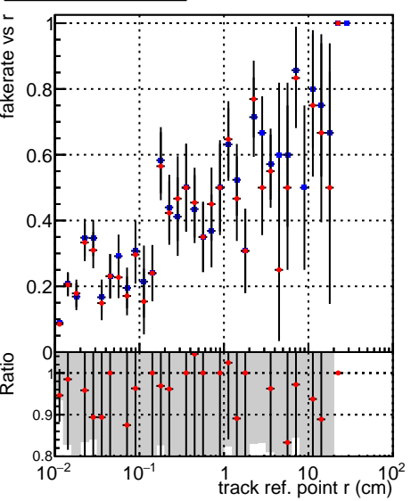
■ DQM_CKF_TTbase ● DQM_CKF_TT_retrainOldFiles125_v2_prelimWP
