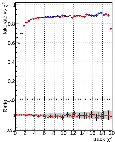
Fake rate vs. —●— DQM_CKF_TTbase —●— DQM_CKF_TT_retrainOldFiles125_v2_prelimWP
