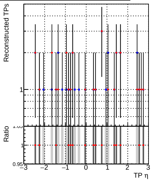
—•— DQM_CKF_TTbase —•— DQM_CKF_TT_retrainOldFiles125_v2_prelimWP
