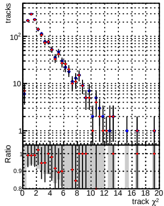
—●— DQM_CKF_TTbase —●— DQM_CKF_TT_retrainOldFiles125_v2_prelimWP
