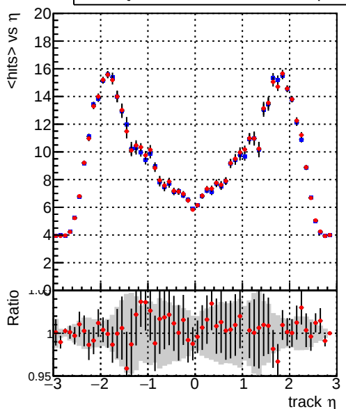
mean hits vs \eta Legend: DQM_CKF_TTbase (blue line), DQM_CKF_TT_retrainOldFiles125_v2_prelimWP (red line)
