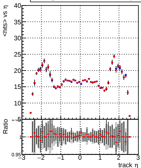
mean hits Legend: DQM_CKF_TTbase (blue line), DQM_CKF_TT_retrainOldFiles125_v2_prelimWP (red line)
