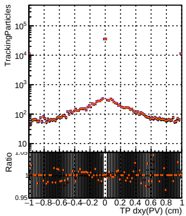
Legend for N of simulated tracks: DQM_mkFit_TTbase DQM_mkFit_TT_retrainOldFiles125_v2_prelimWP_5iter DQM_mkFit_TT_baseline_6iter DQM_mkFit_TT_RetrainV2_WP1_6iter
