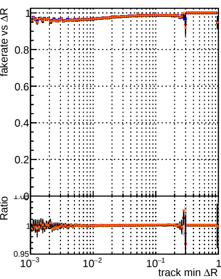
Fake rate vs \Delta R(\text{track, jet}) DOM mkFit Tbase DOM mkFit + RetrainOldFiles125_v2_prelimWP_5iter DOM mkFit + RetrainV2_WP1_6iter
