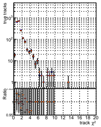
N of reco track vs. \chi^2 for various algorithms: BGM, mREK, REK, REK+, Retrain v2, WP1, 6iter, Retrain Old Files, 125_v2, prelimWP_5iter
