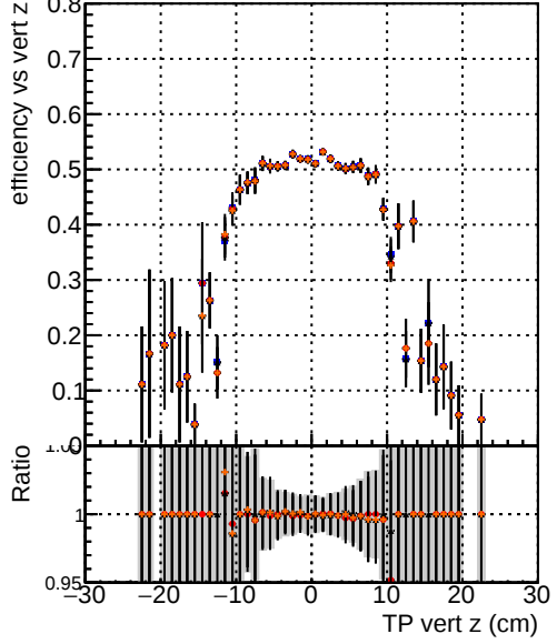
Efficiency vs. sim PV z —●— DQM_mkFit_TTbase —●— DQM_mkFit_TT_retrainOldFiles125_v2_prelimWP_5iter —●— DQM_mkFit_TT_baseline_6iter —●— DQM_mkFit_TT_RetrainV2_WP1_6iter
