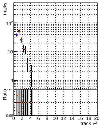
N of reco track vs. \chi^2 Base BSM mFit 125 v2 Prelim WP 5iter BSM mFit 125 v2 Prelim WP 5iter BSM mFit 125 v2 Prelim WP 5iter
