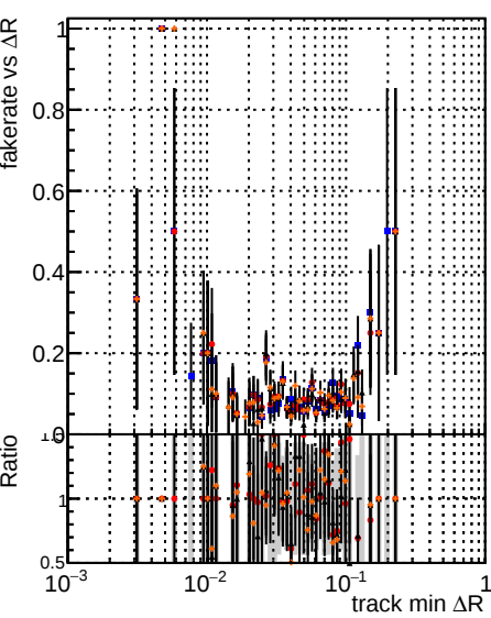
Fake rate vs \Delta R(\text{track, jet}) Legend: DOM mkFit TTbase DOM mkFit TTbaseRetrainOldFiles125_v2_prelimWP_5iter DOM mkFit TTbaseRetrainOldFiles125_v2_prelimWP_5iter DOM mkFit TTbaseRetrainV2_WP1_6iter
