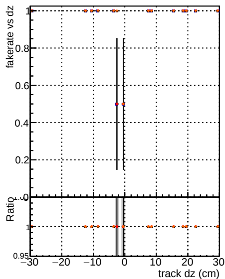
Fake rate vs d DOM mkFit TTbase RetrainOldFiles125_v2_prelimWP_5iter baseLine 5iter Retrainv2 WP1 6iter
