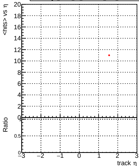
Legend: DQM_mkFit_TTbase (blue line), DQM_mkFit_TT_retrainOldFiles125_v2_prelimWP_5iter (red line with dots), DQM_mkFit_TT_baseline_6iter (black line), DQM_mkFit_TT_RetrainV2_WP1_6iter (orange line) mean hit
