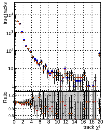
DOM mklfit TTbase DOM mklfit TT RetrainOldFiles125_v2_prelimWP_5iter DOM mklfit TT baseline 5iter DOM mklfit TT RetrainV2 WP1 6iter
