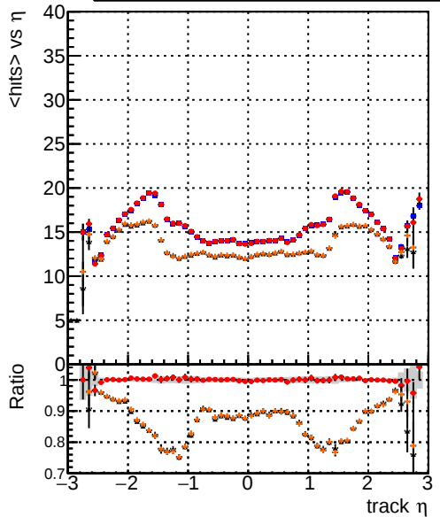
Legend: DQM_mkFit_TTbase (blue), DQM_mkFit_TT_retrainOldFiles125_v2_prelimWP_5iter (red), DQM_mkFit_TT_baseline_6iter (black), DQM_mkFit_TT_RetrainV2_WP1_6iter (orange) mean hits
