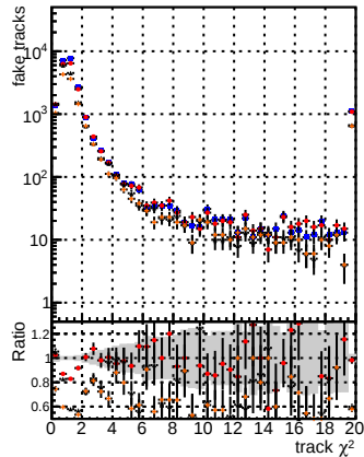
Legend for fake_tracks vs. \chi^2 :
