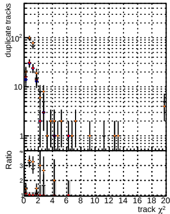
Legend for duplicate_tracks vs. \chi^2 :
