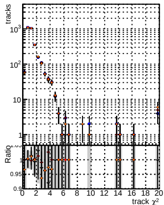
N of reco track vs. \chi^2 for BSM mFit, BSM mFit + Retrain v2, WP1, WP1 5iter, Retrain v2 WP1 5iter
