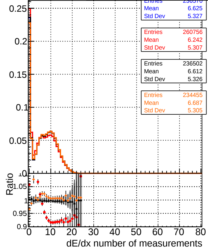
Legend for bottom row: DQM_mkFit_TTbase (Blue line) DQM_mkFit_TT_retrainOldFiles125_v2_prelimWP_5iter (Red line) DQM_mkFit_TT_baseline_6iter (Black line) DQM_mkFit_TT_RetrainV2_WP1_6iter (Orange line)
