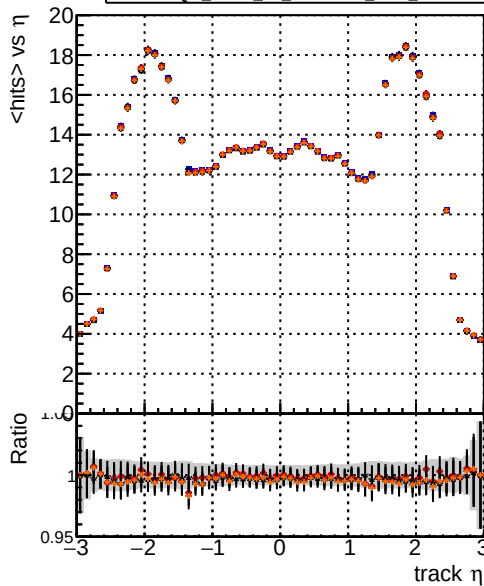
Legend: DQM_mkFit_TTbase (blue line), DQM_mkFit_TT_retrainOldFiles125_v2_prelimWP_5iter (red line), DQM_mkFit_TT_baseline_6iter (black line), DQM_mkFit_TT_RetrainV2_WP1_6iter (orange line) mean hits
