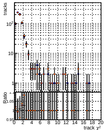
N of reco track vs. \chi^2 for various models: BSM mktFit, BSM mktFit + base, BSM mktFit + base + 125_v2_prelimWP_5iter, BSM mktFit + base + 125_v2_prelimWP_5iter + Refrain v2_WP1_6iter
