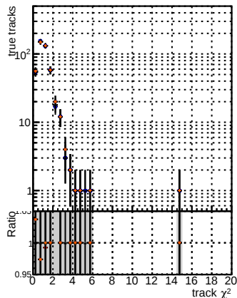
N of reco track vs. \chi^2 for various models: BSM mktFit, BSM mktFit + base, BSM mktFit + base + 125_v2_prelimWP_5iter, BSM mktFit + base + 125_v2_prelimWP_5iter + Refrain v2_WP1_6iter
