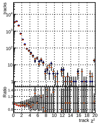
N of reco track vs. \chi^2 for BSM mktFit + base + old files + 125 v2 prelinWP_5iter
