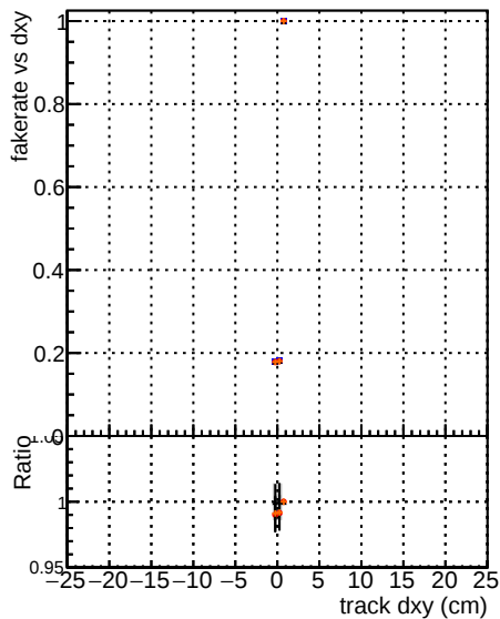
Fake rate vs d DOM mkFit TTbase retrainOldFiles125_v2_prelimWP_5iter baseline_6iter retrainv2 WP1_6iter
