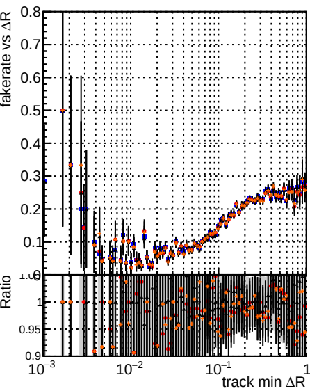
Fake rate vs \Delta R(\text{track, jet}) Legend: DOM mkFit TTbase RetrainOldFiles125_v2_prelimWP_5iter DOM mkFit TTbase RetrainOldFiles125_v2_prelimWP_5iter DOM mkFit TTbase RetrainOldFiles125_v2_prelimWP_5iter
