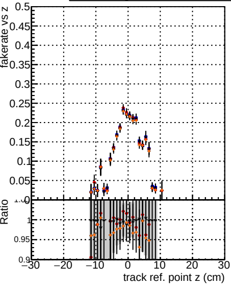
Fake rate vs v DOM mktFit Tbase RetrainOldFiles125_v2_prelimWP_5iter DOM mktFit Tbase RetrainOldFiles125_v2_prelimWP_5iter DOM mktFit Tbase RetrainV2 WP1 6iter
