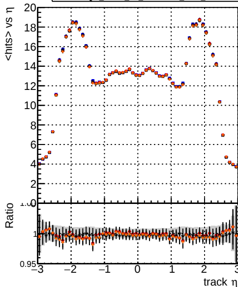
mean hits vs \eta Legend: DOM_mkFit_TTbase DOM_mkFit_TT_retrainOldFiles125_v2_prelimWP_5iter DOM_mkFit_TT_baseline_6iter DOM_mkFit_TT_RetrainV2_WP1_6iter
